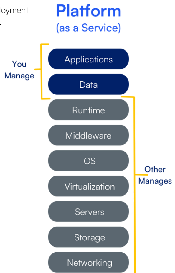
Figure 2 - PaaS Responsibilities
