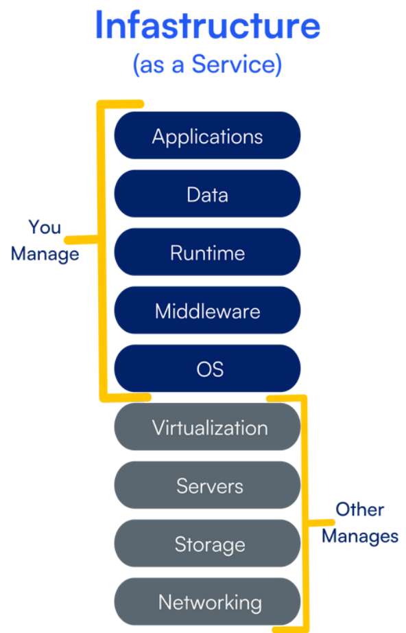
Figure 1 - IaaS Responsibilities
